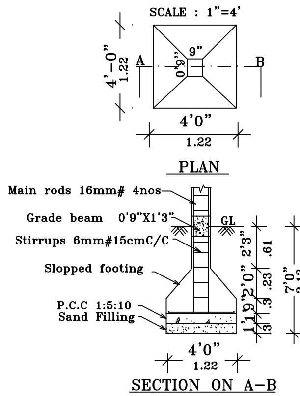
COLUMN DETAILS
