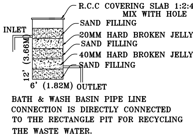
WASTE WATER RECYCLE UNIT
