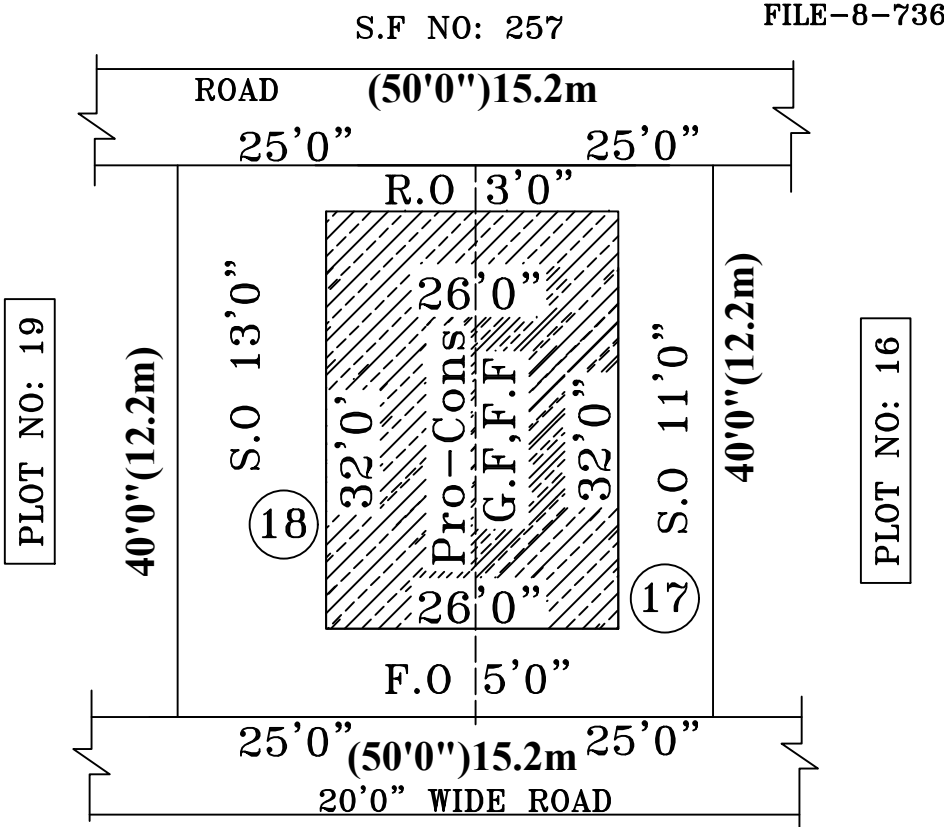
SITE PLAN
