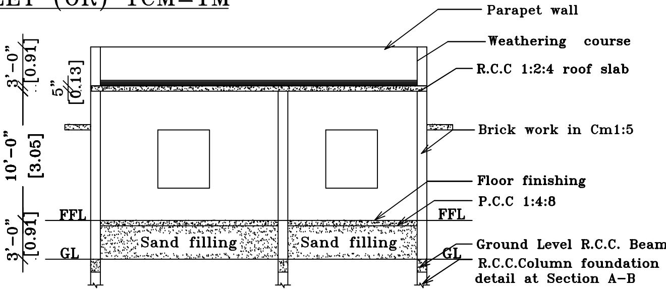
SECTION ON 'SJ'
