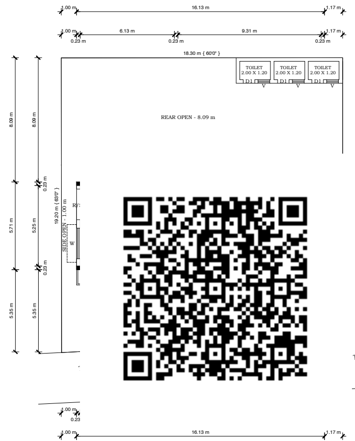
PROPOSED BASEMENT FLOOR PLAN
