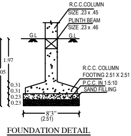
FOUNDATION DETAIL
