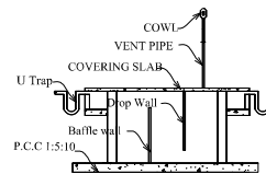
SECTION ON JS1
