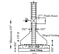
ISOLATED FOOTING / COLUMN DETAIL
