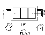
F FLOOR PLAN
