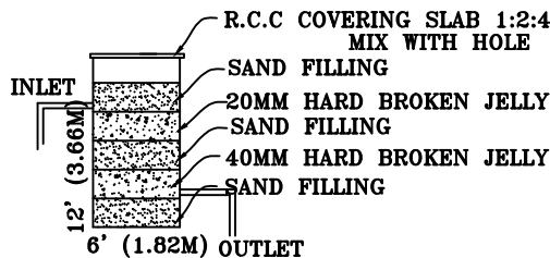
WASTE WATER RECYCLE UNIT
