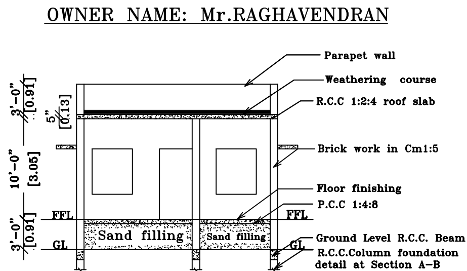
SECTION ON 'SJ'
