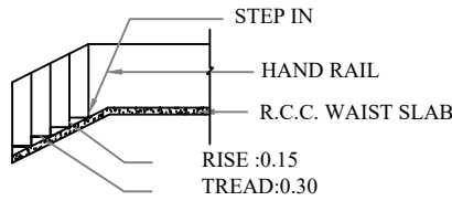
STAIR DETAILS
