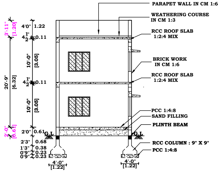
SECTION - KK
