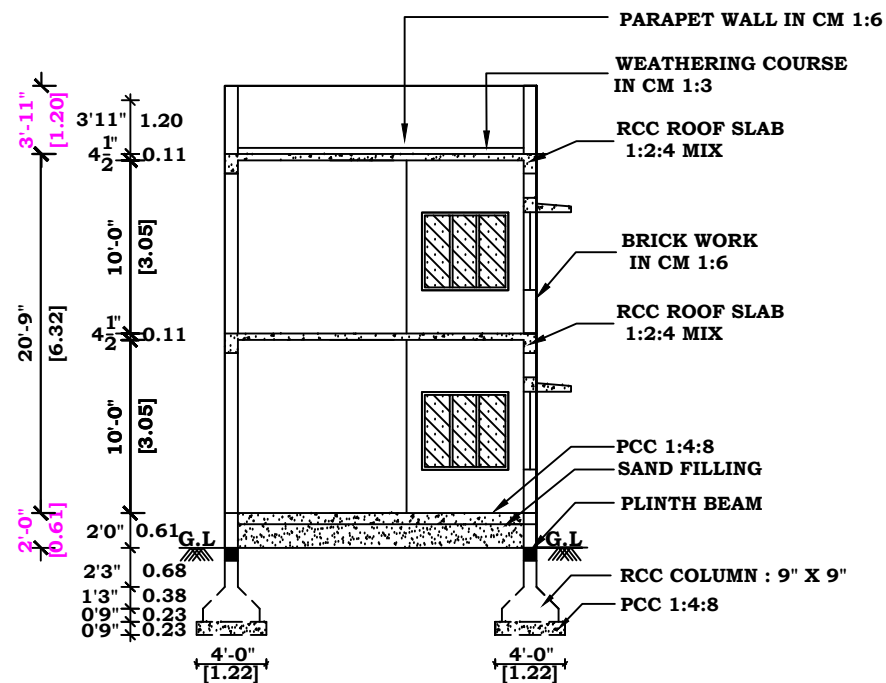
SECTION - KK
