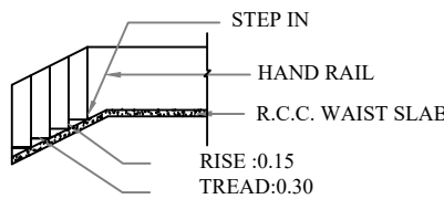
STAIR DETAILS
