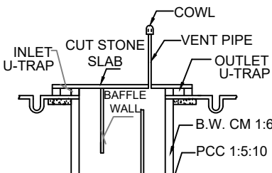
SEPTIC TANK DETAILS SIZE :6'0" x 3'0" x 6'0"
