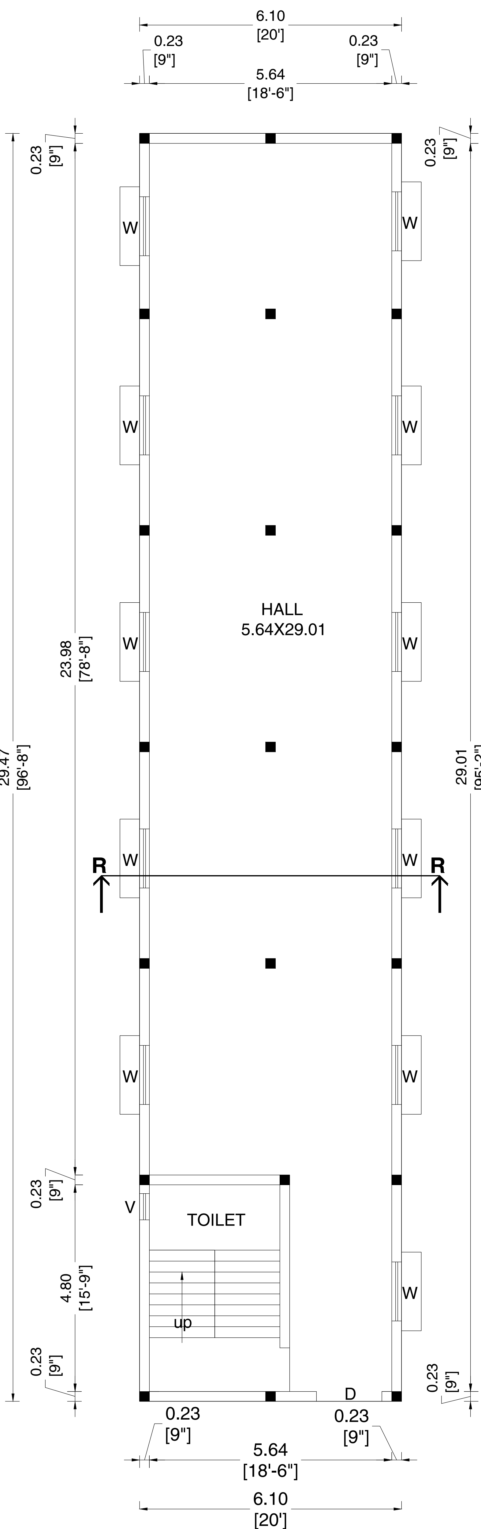
PRO. GROUND FLOOR PLAN
