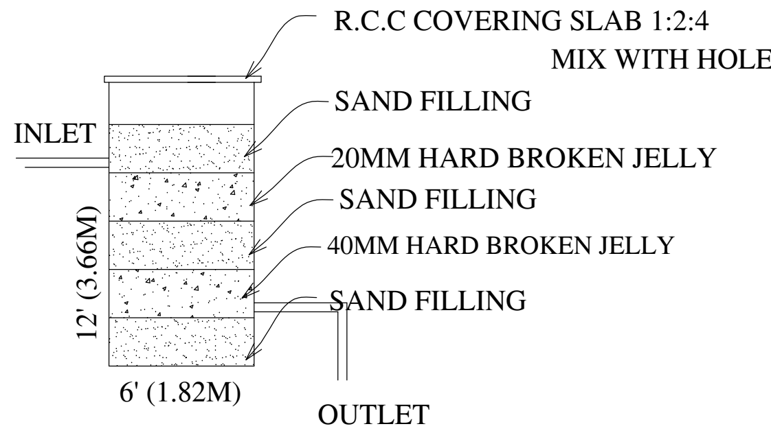
Waste Water Recycle Unit Not To Scale
