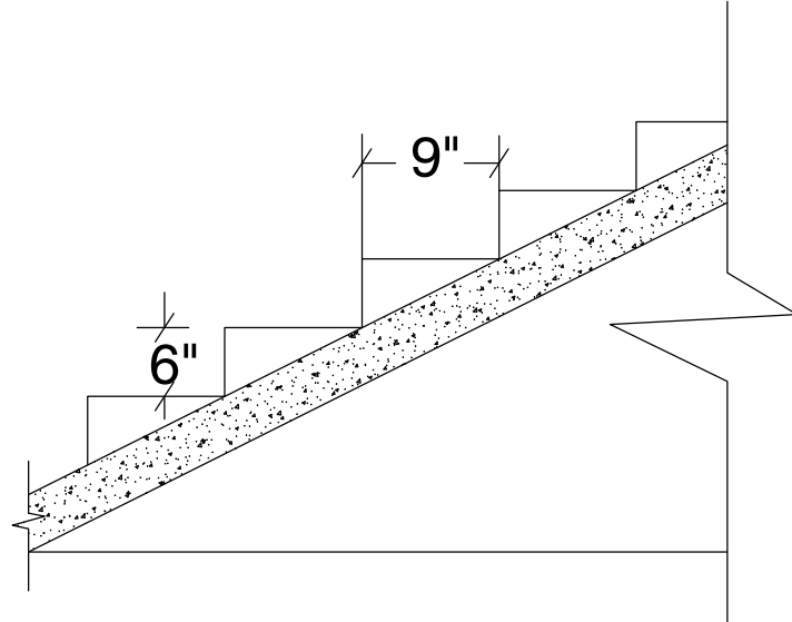
Staircase Detail Not To Scale NOTE: Width - 3'0" - 0.91M Tread - 0'9" - 0.23M Rise - 0'6" - 0.15M
