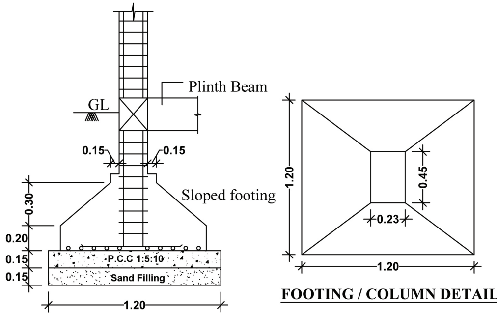
ISOLATED FOOTING / COLUMN DETAIL
