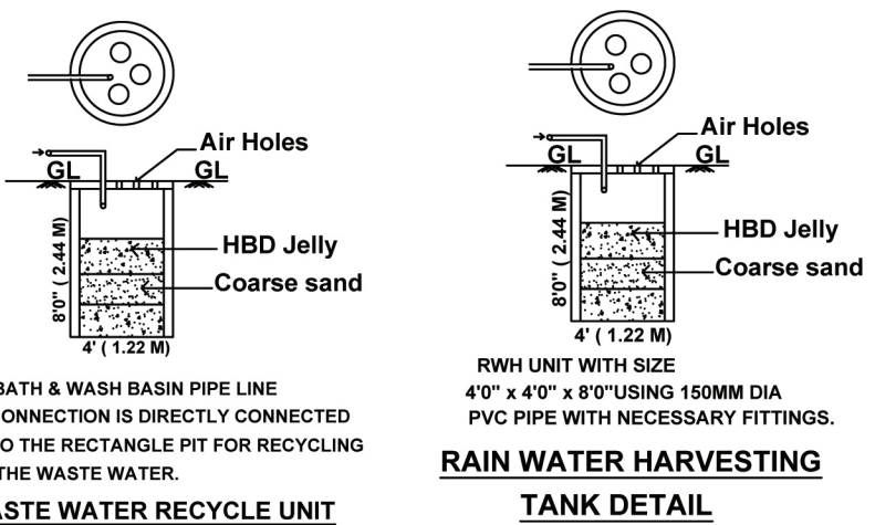
WASTE WATER RECYCLE UNIT
