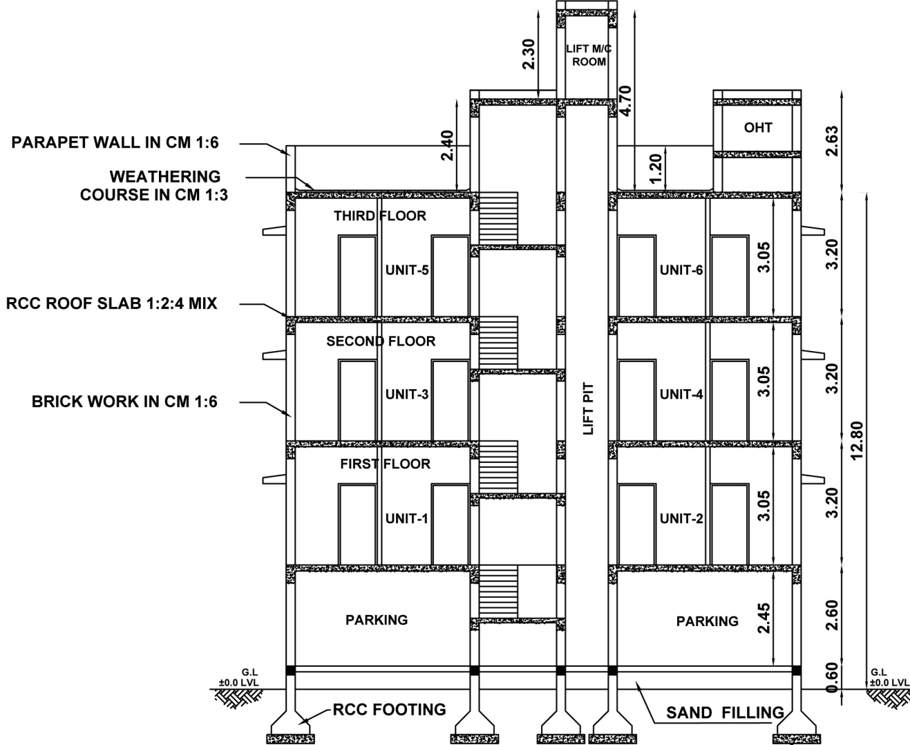
SECTION-AA
