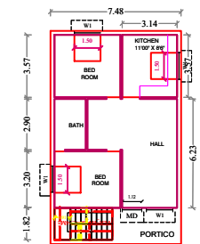
EXISTING GROUND FLOOR
