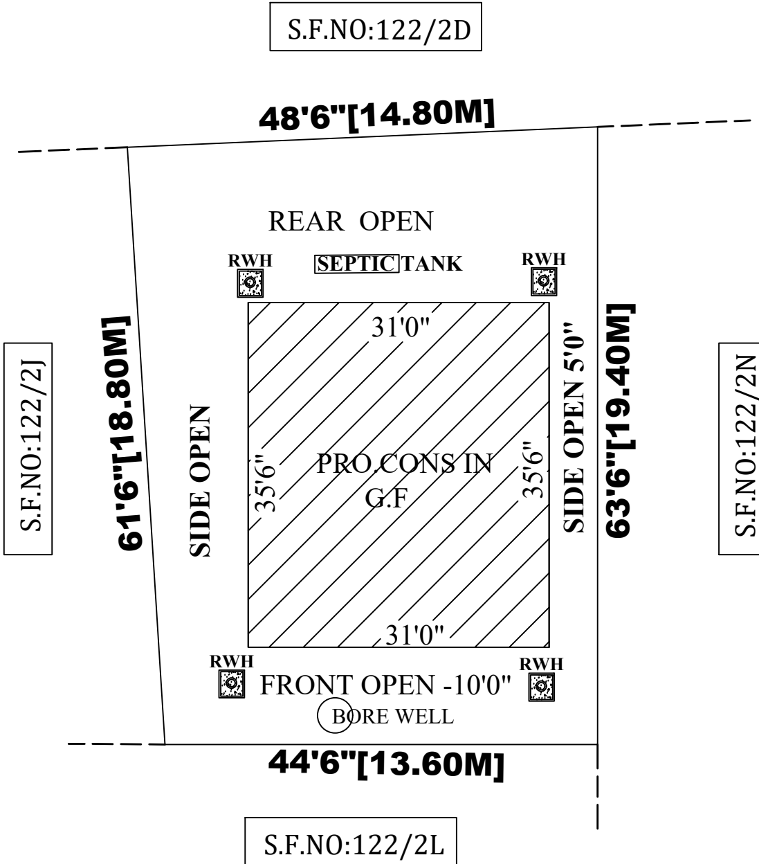
SITE PLAN
