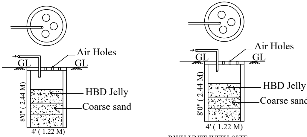
RAIN WATER HARVESTING TANK DETAIL
