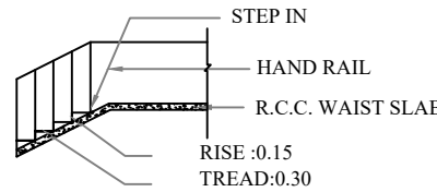
STAIR DETAILS
