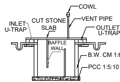
SEPTIC TANK DETAILS SIZE : 6'0" x 3'0" x 6'0"
