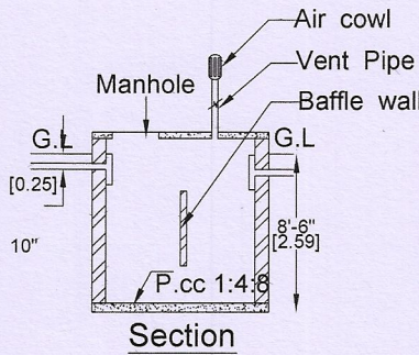
RAINWATER HARVESTING TANK SCALE 1:50
