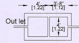
Plan SEPTIC TANK DETAIL
