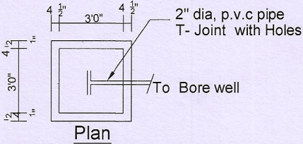
RAINWATER HARVESTING TANK SCALE 1:50
