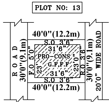
SITE PLAN
