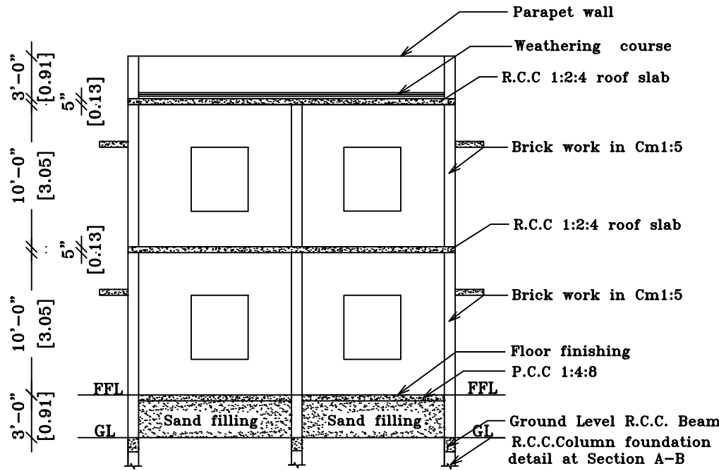
SECTION ON 'SK'
