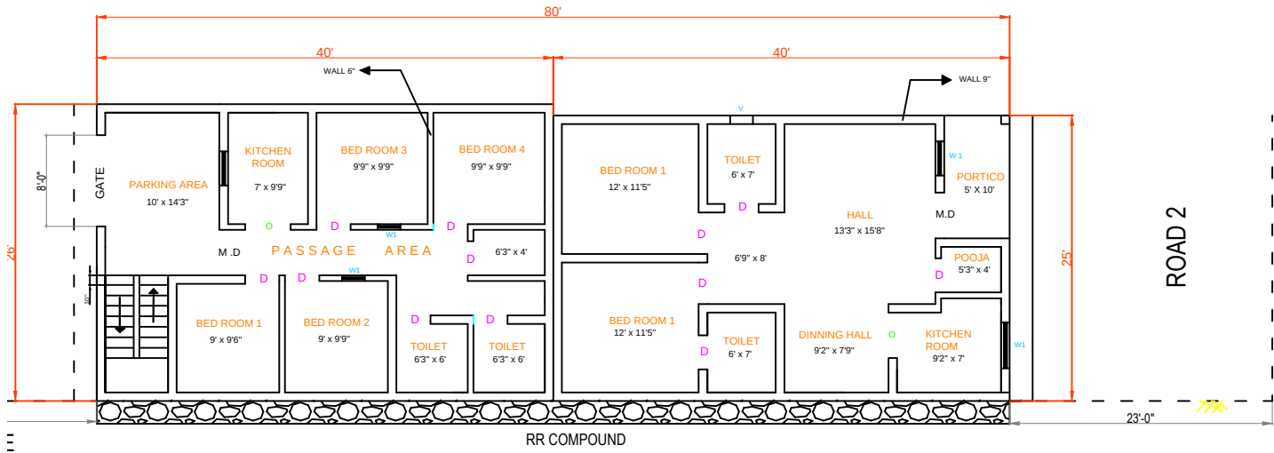
GROUND FLOOR
