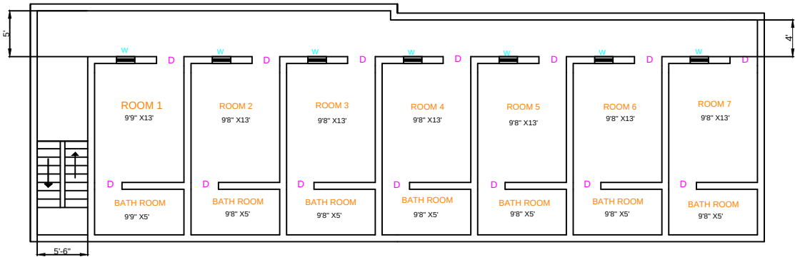
FIRST FLOOR
