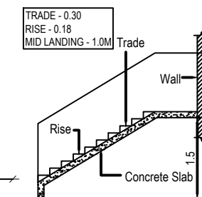
STAIR DETAILS
