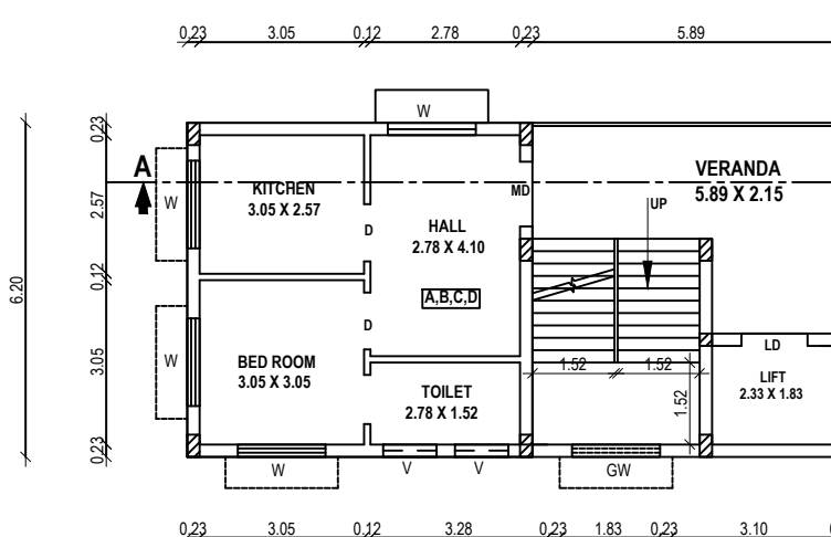
PRO TYPICAL FIRST, SECOND, THIRD, FOURTH FLOOR PLAN
