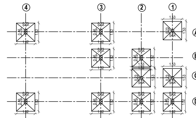
COLUMN POSITION PLAN
