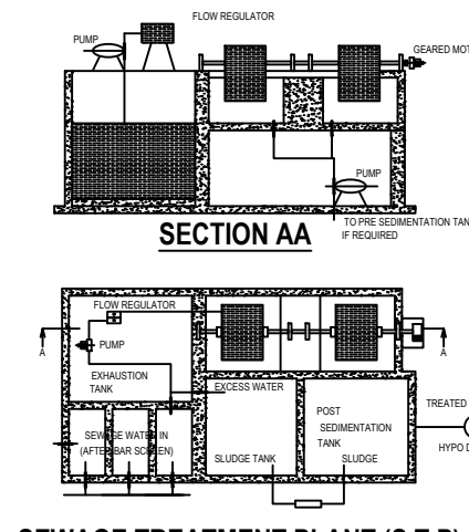
SEWAGE TREATMENT PLANT (S.T.P.)
