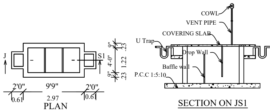
SECTION ON JS1
