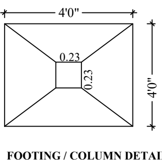
FOOTING / COLUMN DETAIL
