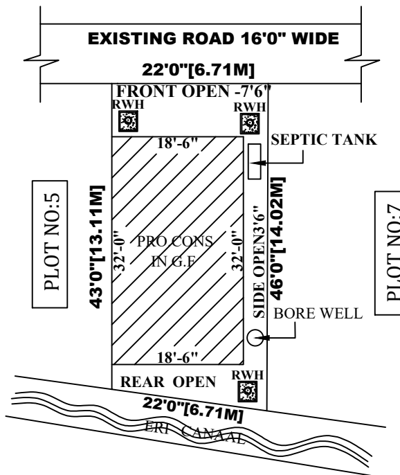
SITE PLAN
