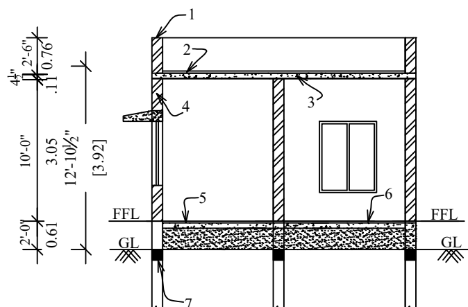
FOUNDATION DETAIL DESIGNED AS PER LOCAL SOIL CONDITION
