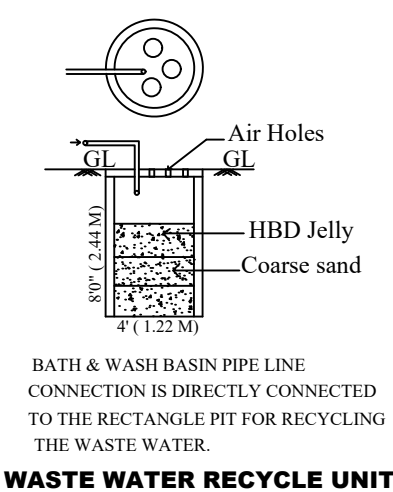
WASTE WATER RECYCLE UNIT
