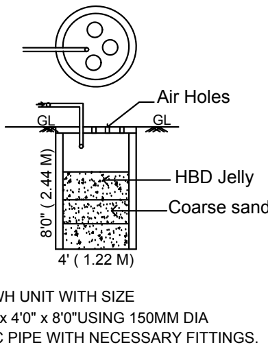
RAIN WATER HARVESTING TANK DETAIL
