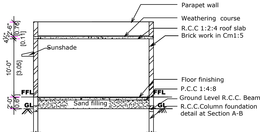
SECTION ON 'RK'
