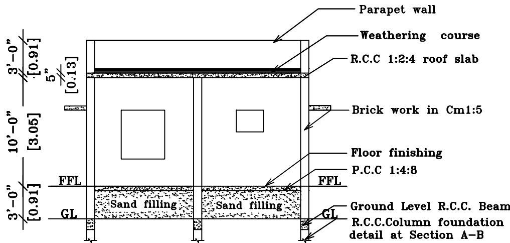
SECTION ON 'SJ'
