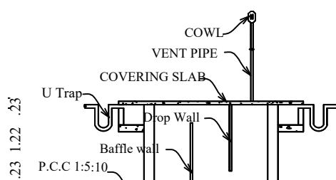
SECTION ON JS1
