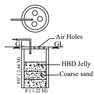
WASTE WATER RECYCLE UNIT
