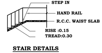
STAIR DETAILS
