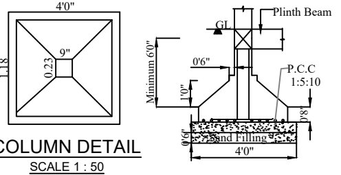
RAINWATER HARVESTING UNIT RWHL SIZE :4'0" X 4'0" X 10'0" - 3 NOS USING 150MM PIPE AND NECESSARY SPECIALS.
