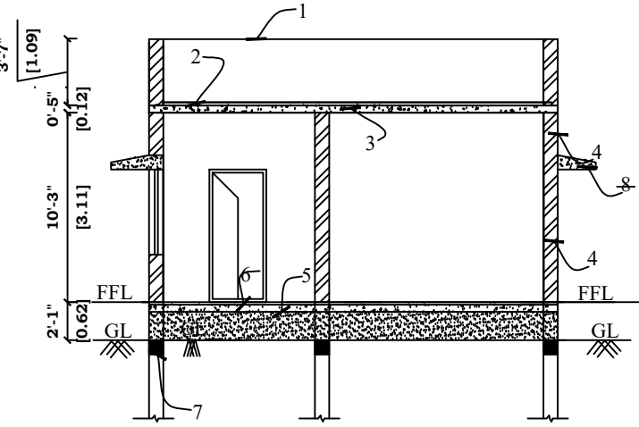
FOUNDATION DETAIL DESIGNED AS PER LOCAL SOIL CONDITION SECTION AA'
