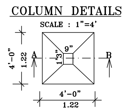
PLAN
