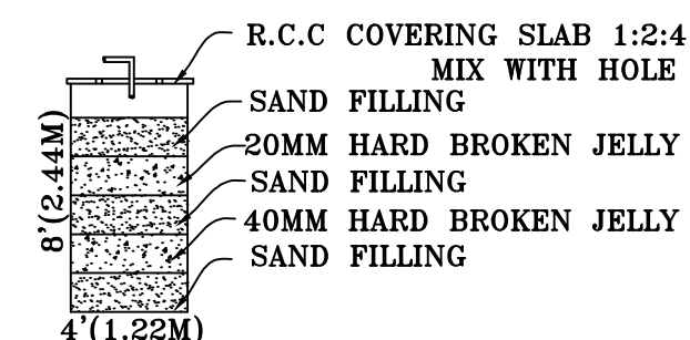
RAIN WATER HARVEST UNIT
