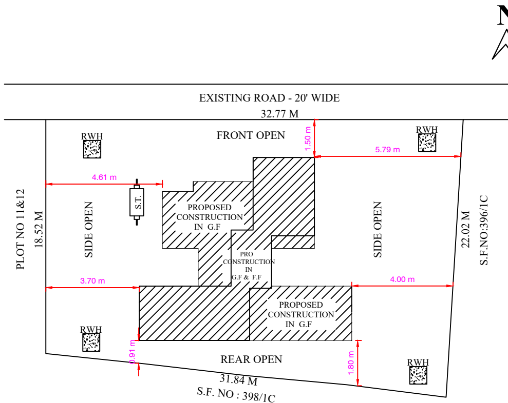
SITE PLAN
