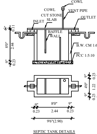
SEPTIC TANK DETAILS
