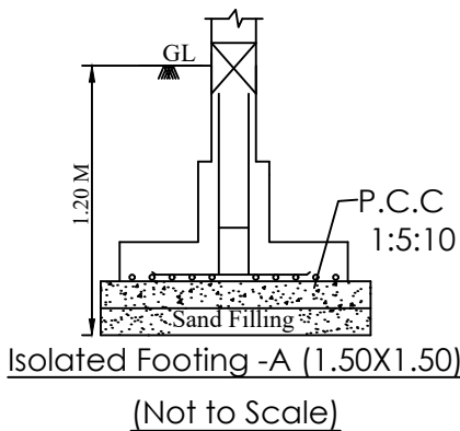
Isolated Footing - A (1.50X1.50)
