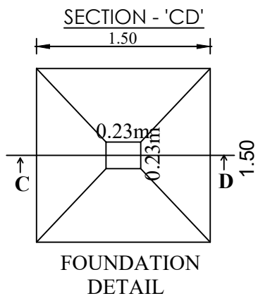
Isolated Footing - A (1.50X1.50)
