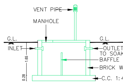
SECTION OF SEPT. TANK
