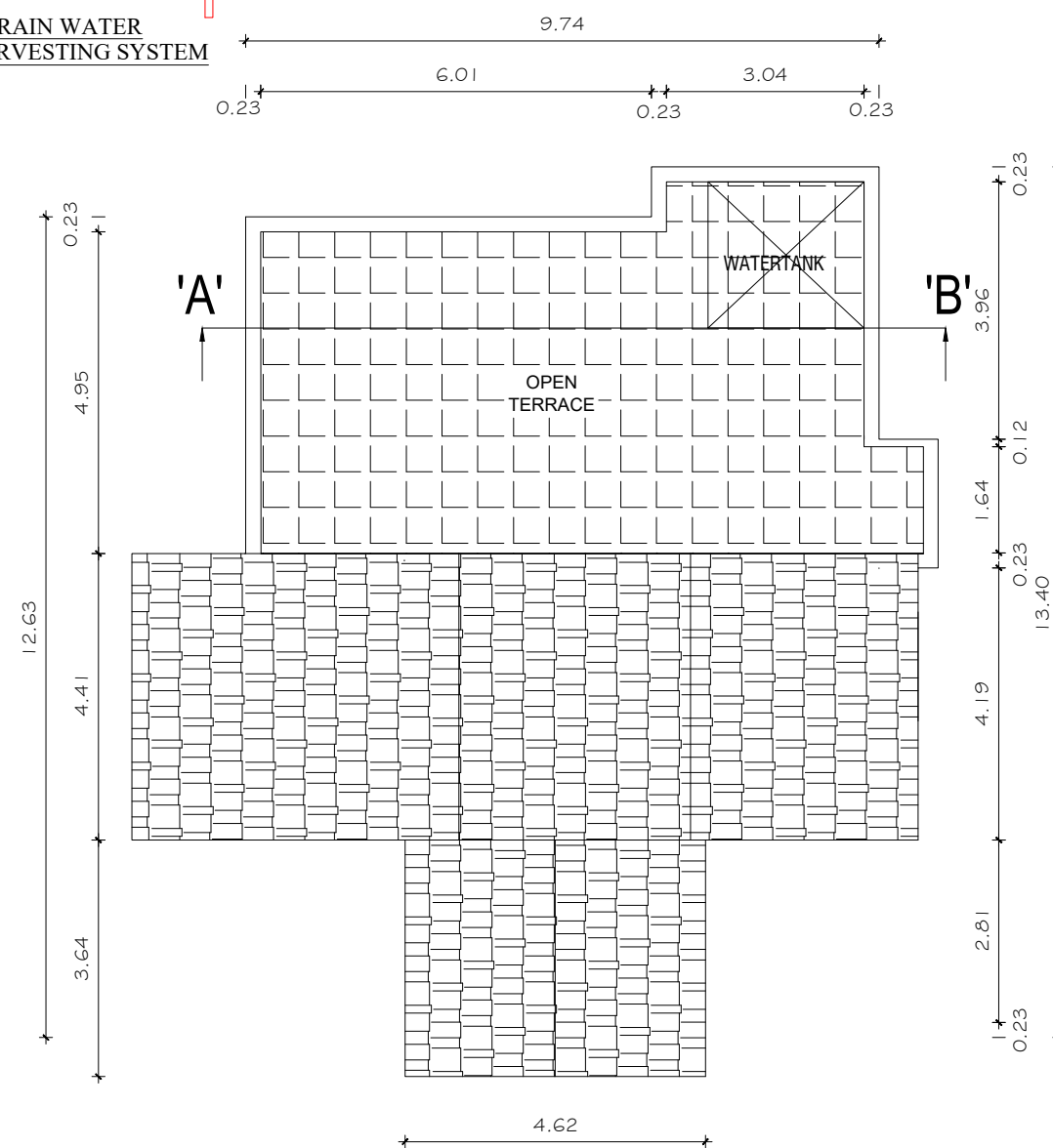
PRO. TERRACE FLOOR PLAN.
