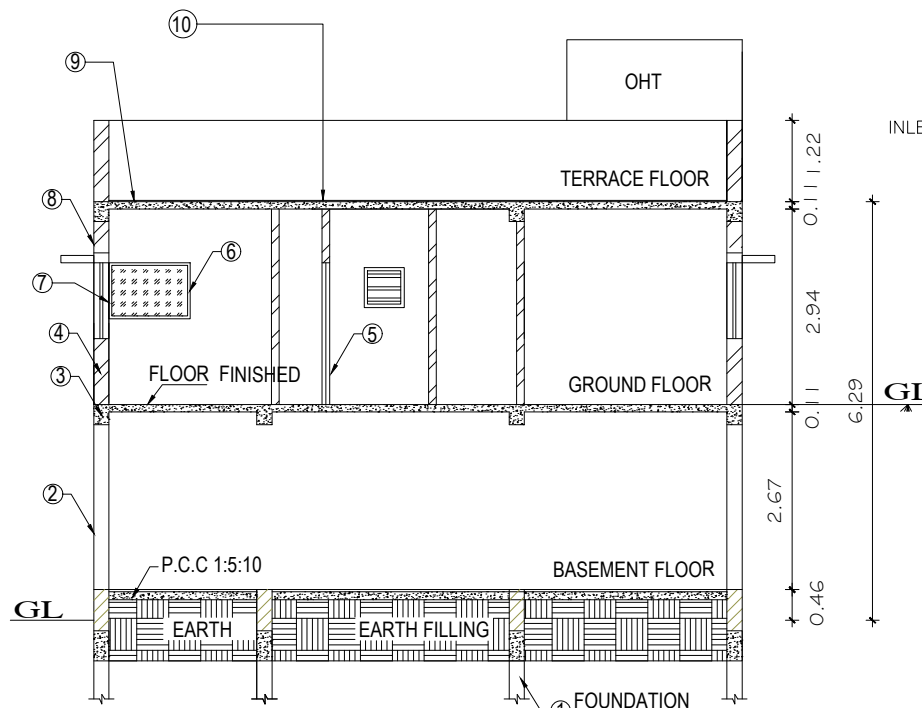
SECTION "A-B"
