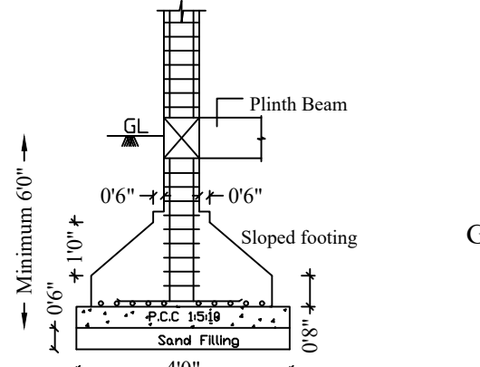
ISOLATED FOOTING / COLUMN DETAIL
