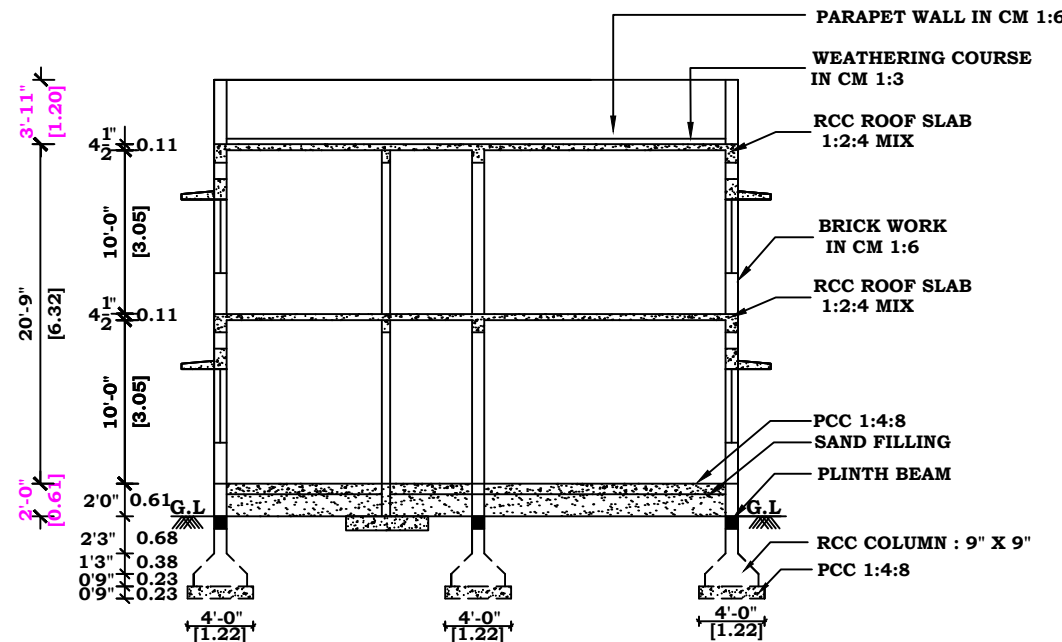
SECTION - KK
