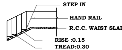
STAIR DETAILS
