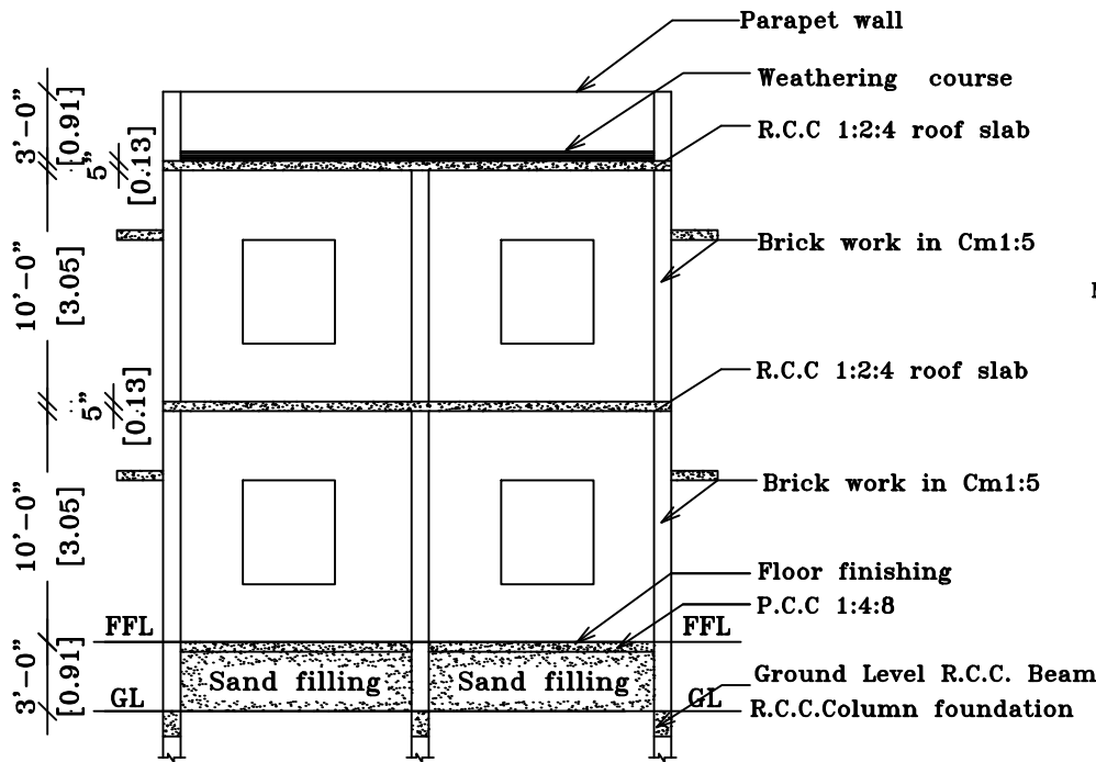
SECTION ON 'SJ'
