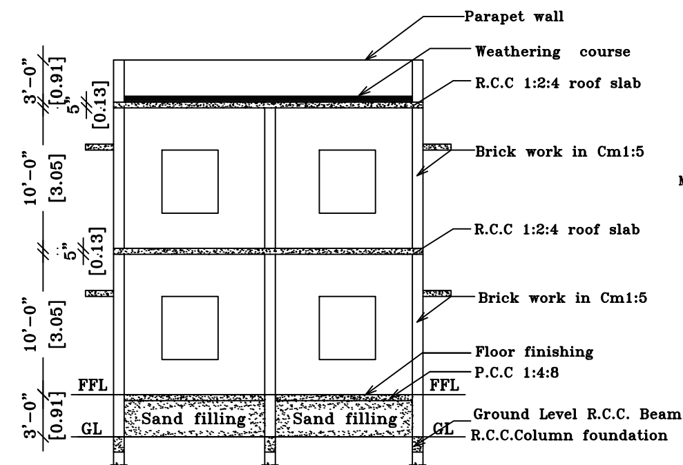
SECTION ON 'SJ'
