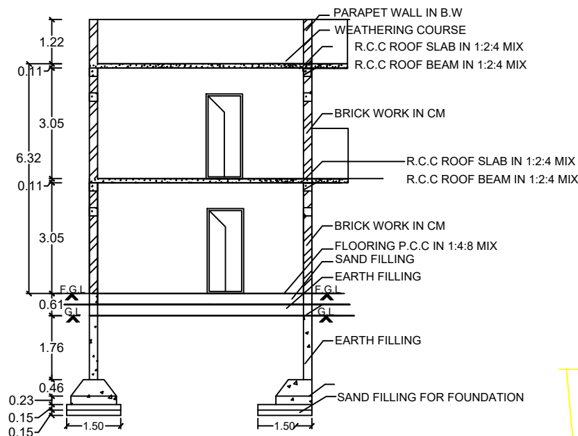
SECTION ON-AA
