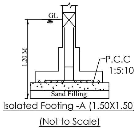
FOUNDATION DETAIL
