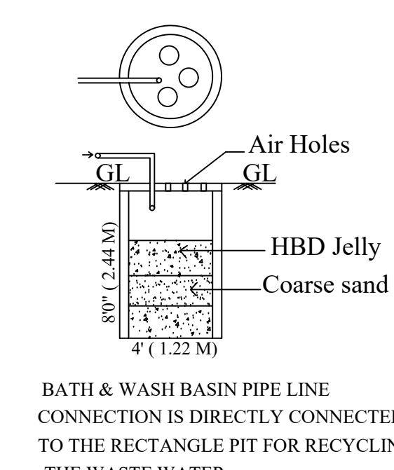
WASTE WATER RECYCLE UNIT
