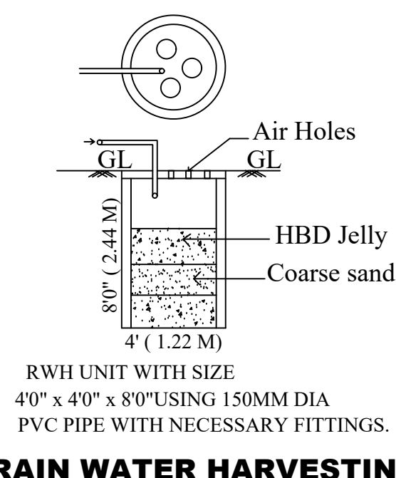
RAIN WATER HARVESTING TANK DETAIL
