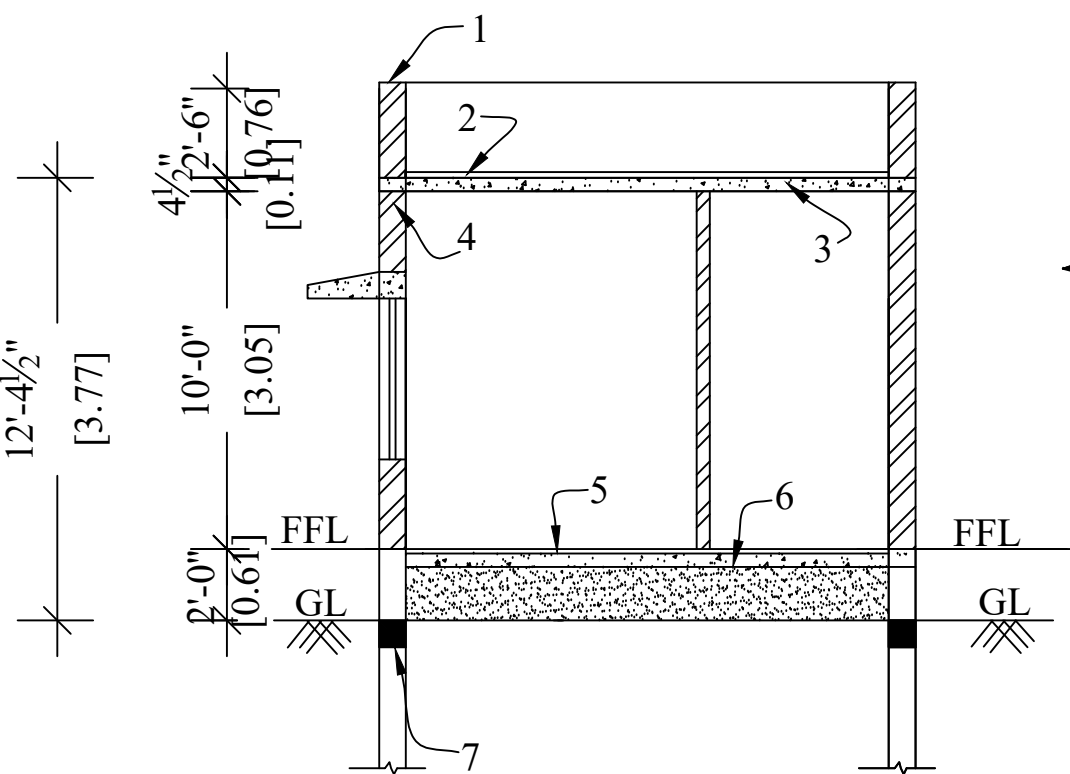
FOUNDATION DETAIL DESIGNED AS PER LOCAL SOIL CONDITION
