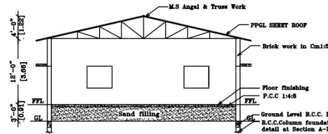
SECTION ON 'SJ'
