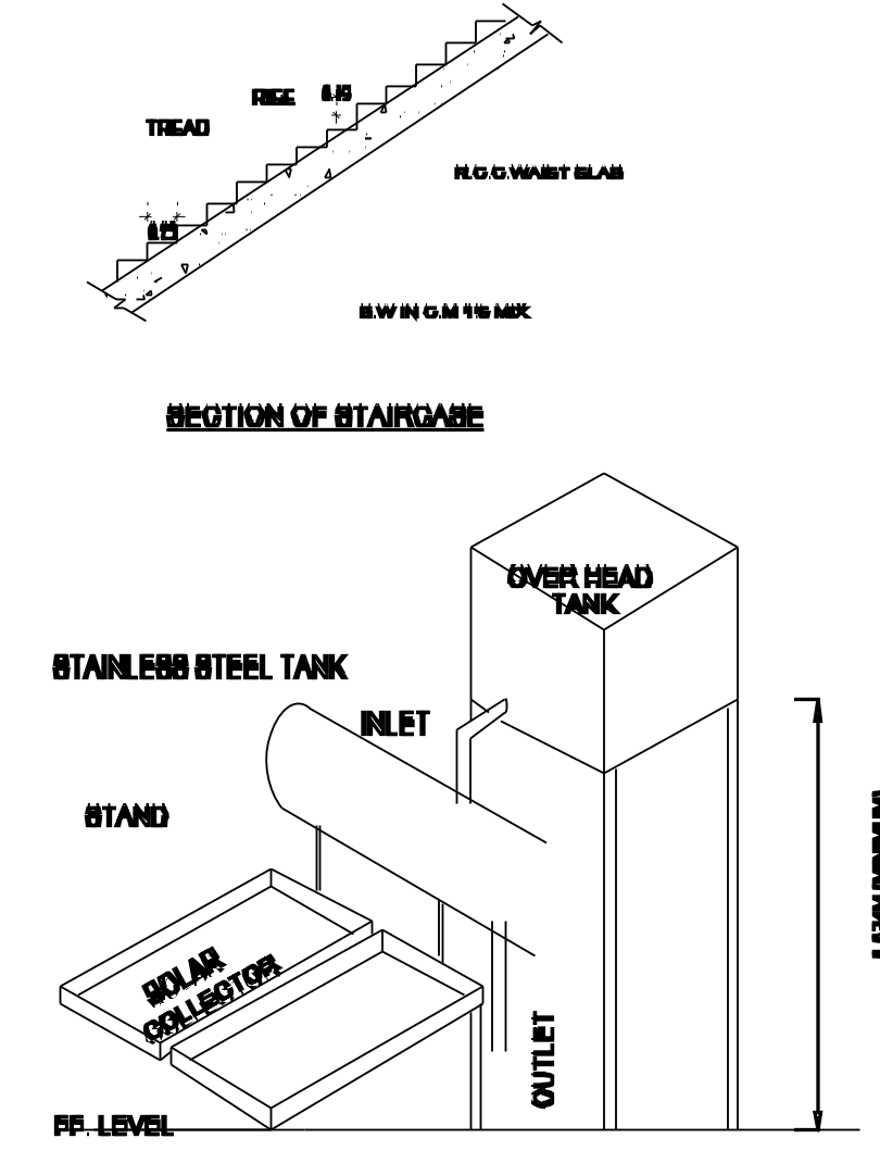
SOLAR WATER HEATING SYSTEM
