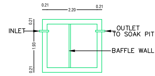
PLAN SEPTIC. TANK (NOT TO SCALE)
