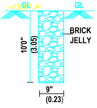
PERCOLATION PIT
