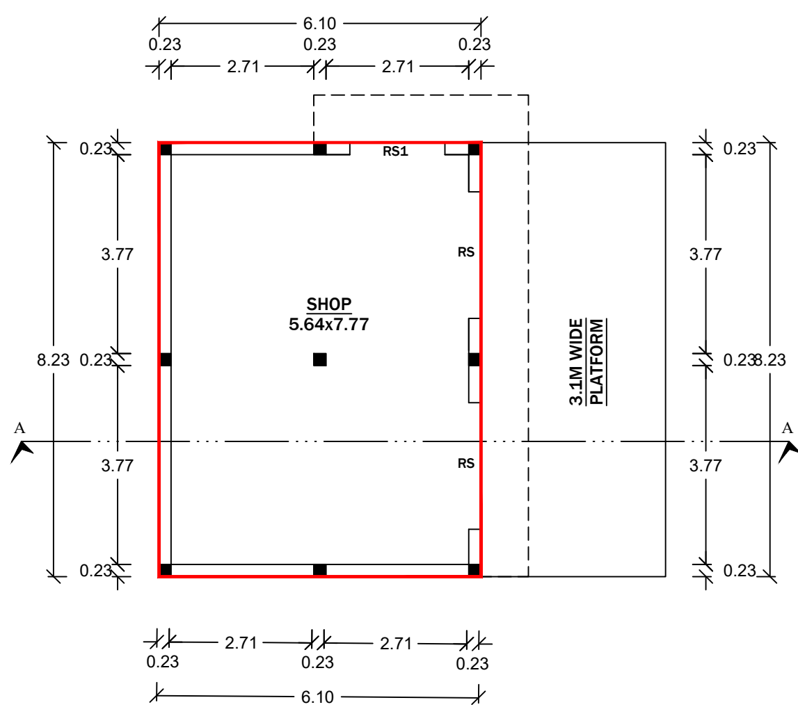
PROPOSED GROUND FLOOR PLAN (GF)
