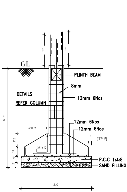
DETAILS TO SCALE)
