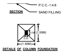
DETAILS OF COLUMN FOUNDATION
