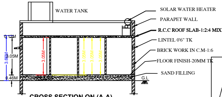
CROSS SECTION ON (A-A)
