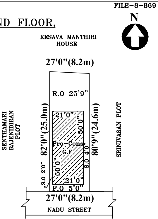
SITE PLAN
