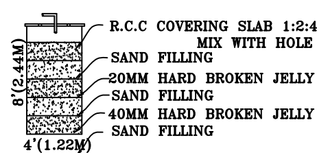
RAIN WATER HARVEST UNIT
