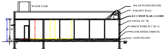
CROSS SECTION ON (A-A)
