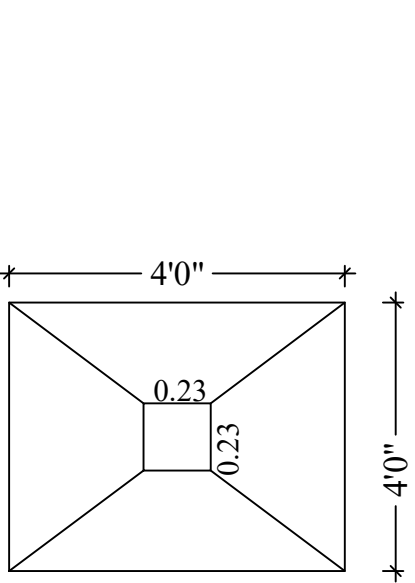
FOOTING / COLUMN DETAIL
