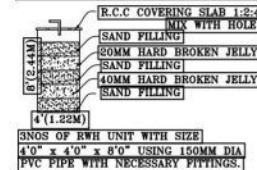
RAIN WATER HARVEST UNIT
