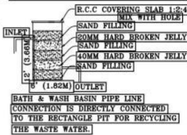
WASTE WATER RECYCLE UNIT
