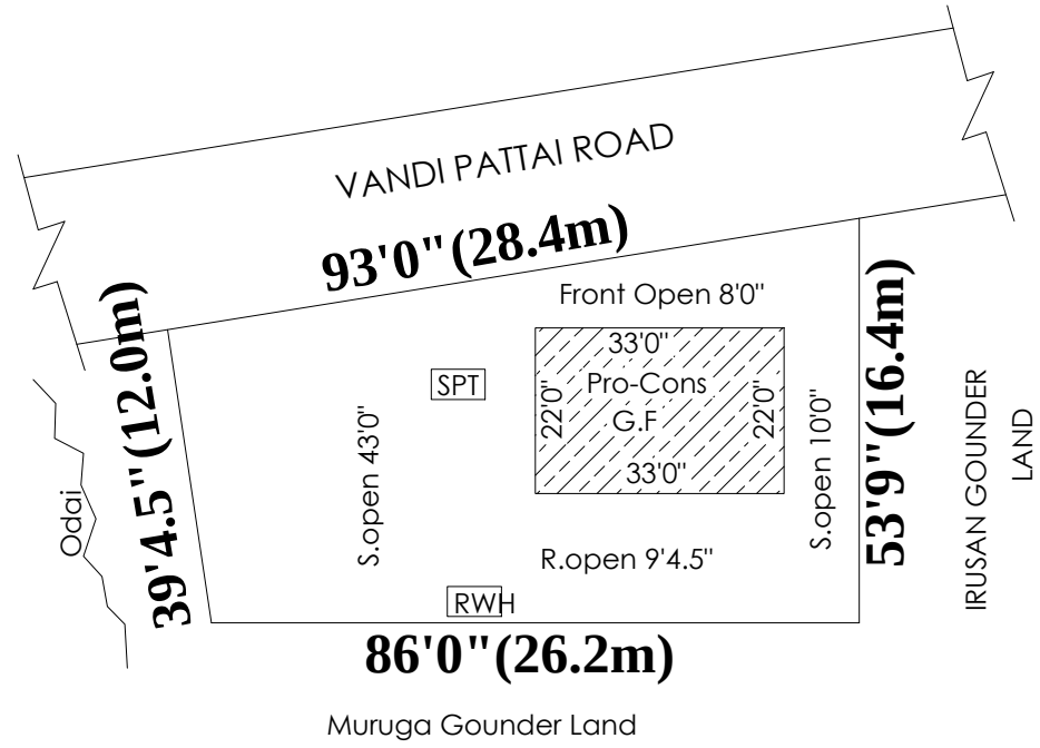
SITE PLAN
