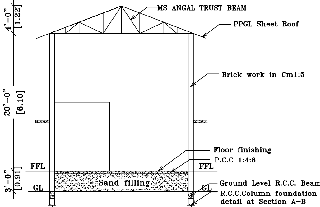
SECTION ON 'SA'
