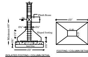
COLUMN DETAILS
