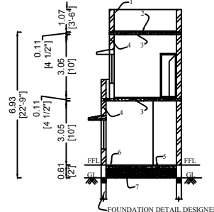
SECTION ON "JS"
