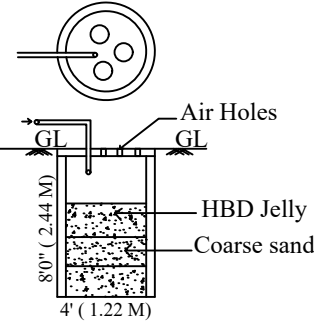
RAIN WATER HARVESTING TANK DETAIL
