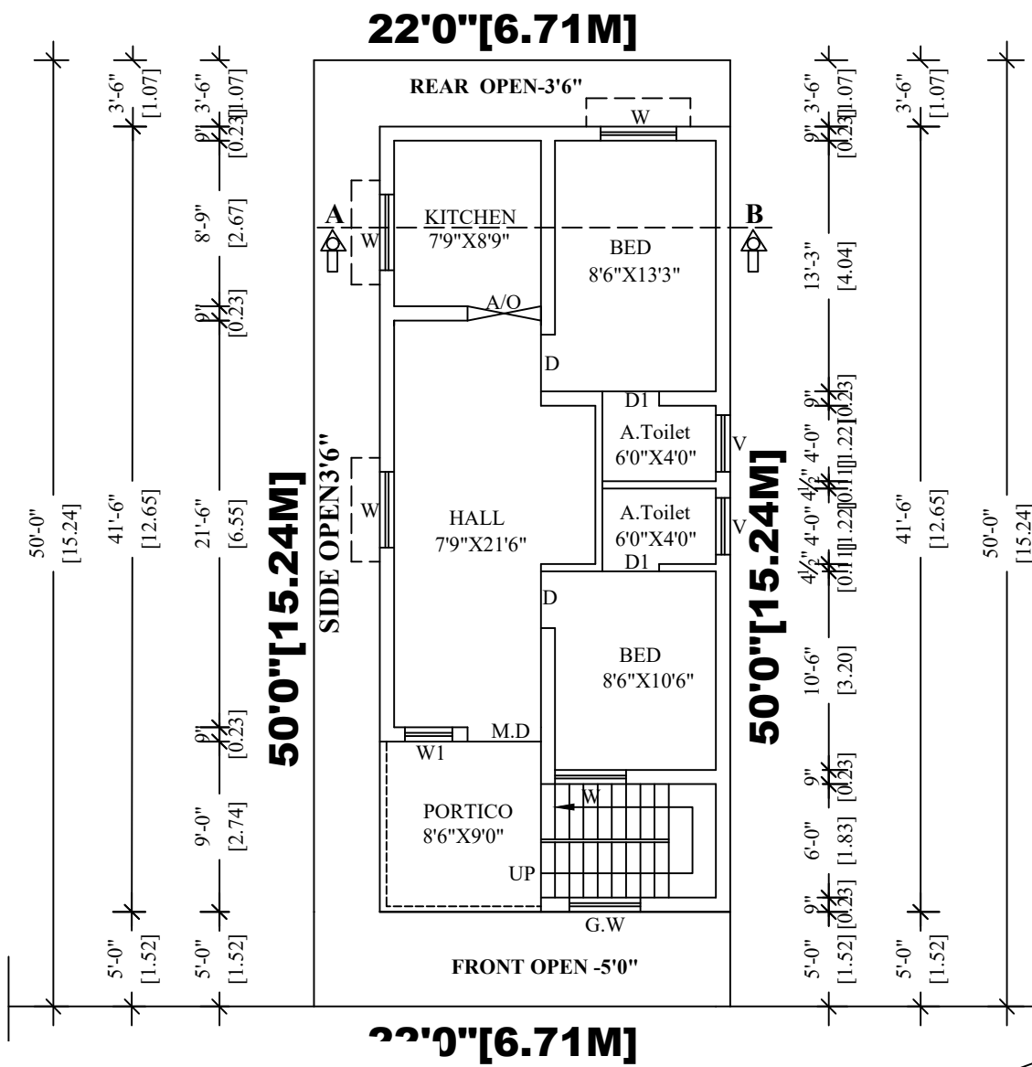
IND FLOOR PLAN
