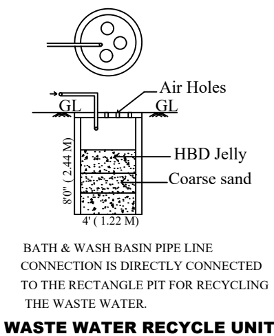
WASTE WATER RECYCLE UNIT
