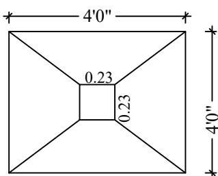
FOOTING / COLUMN DETAIL
