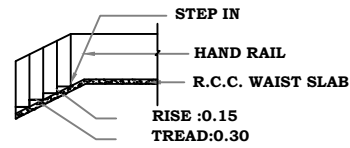
STAIR DETAILS
