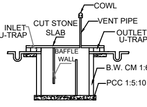
SEPTIC TANK DETAILS SIZE: 6'0" x 3'0" x 6'0"
