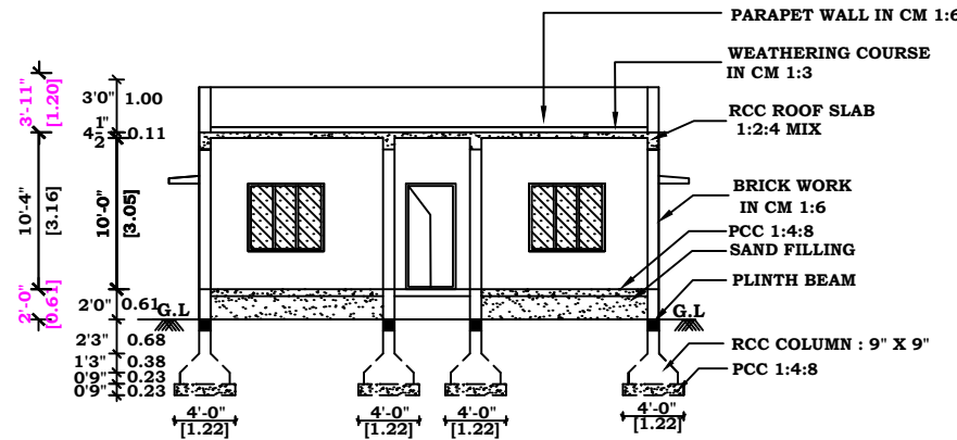
SECTION - KK
