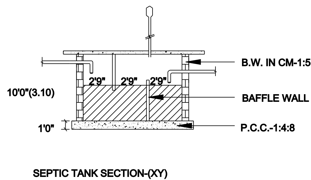
SEPTIC TANK SECTION-(XY)
