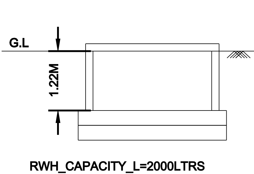
RWH_CAPACITY_L=2000LTRS
