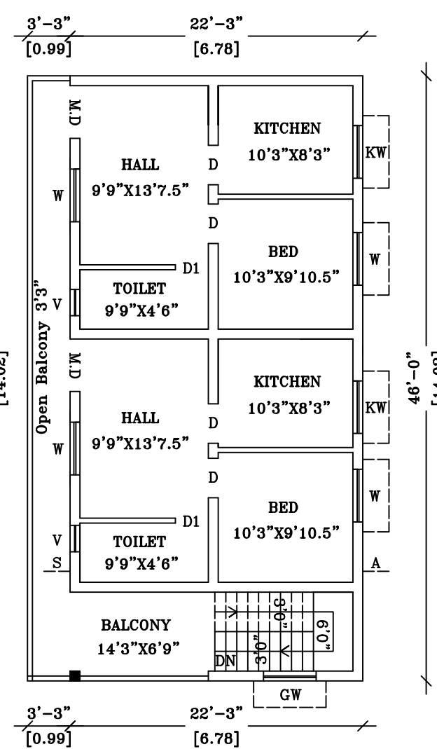
PRO. ADDLCONS FIRST FLOOR PLAN
