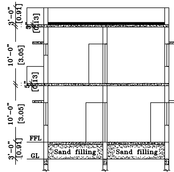
SECTION ON 'SA'
