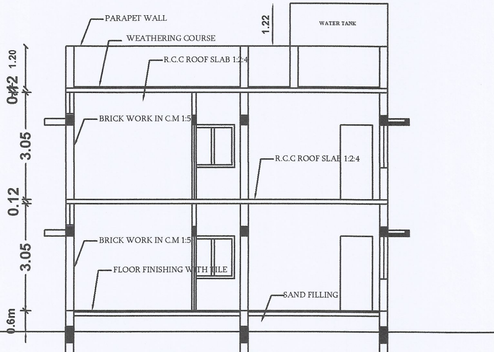
SECTION S-S
