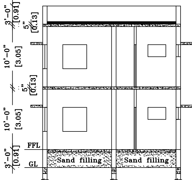
SECTION ON 'SA'
