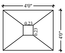
FOOTING / COLUMN DETAIL
