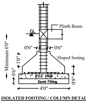
ISOLATED FOOTING / COLUMN DETAIL
