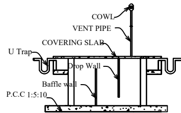
SECTION ON JS1
